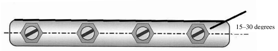
Figure 1 —Spray Bar Nozzle Orientation in Spray Bar
